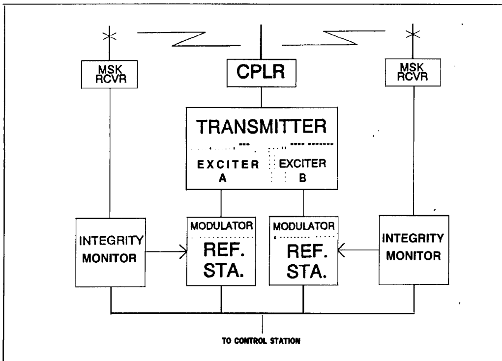
Figure 8. - BROADCAST SITE DIAGRAM
