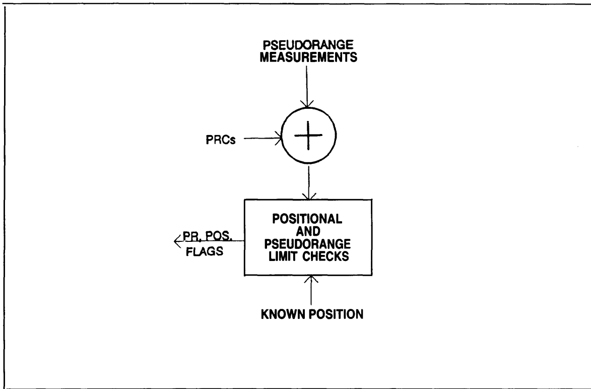
FIGURE 9.- INTEGRIH MONITOR PROCESS
